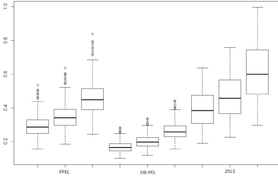
Figure 2. Width of 90% (left), 95% (middle), and 99% (right) CI for \beta_x estimated by PPEL, DB-PEL, and 2SLS under moderate correlation between \epsilon_i and w_{3i} with (n, d_w, s) = (100, 120, 8) .
